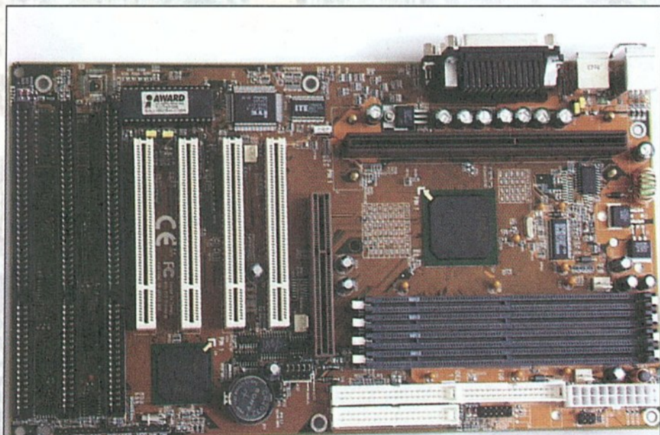
SHUTTLE 637V22
